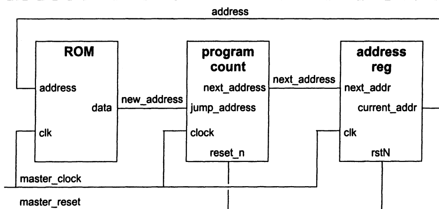
Figure 8-1: Diagram of a simple netlist
