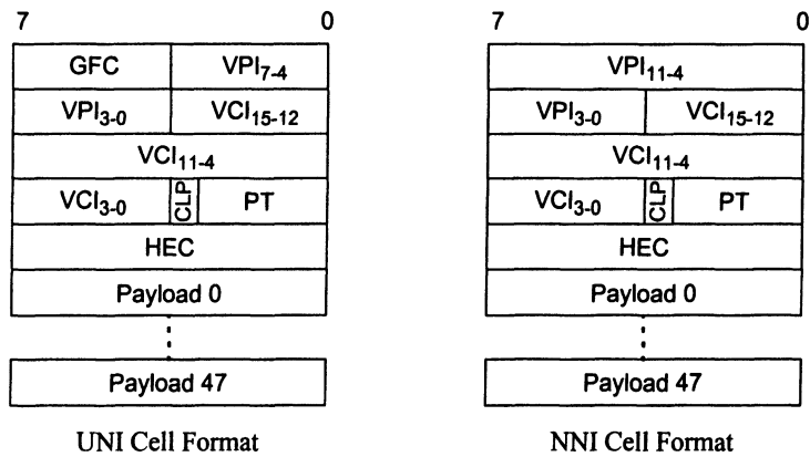
Figure 10-1: UNI and NNI cell formats
