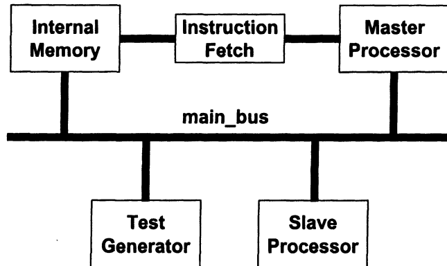
Example 9-1: Verilog module interconnections for a simple design
