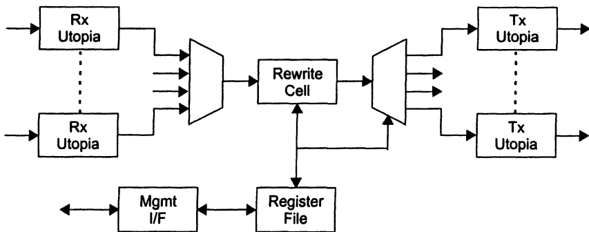
Figure 10-2: Design top-level structural diagram
