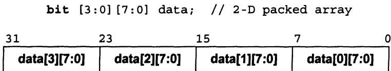
Figure 4-4: Packed arrays are stored as contiguous elements
