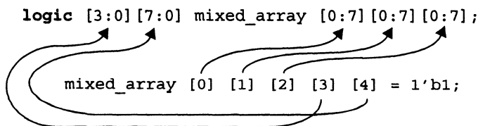
Figure 4-5: Selection order for mixed packed/unpacked multi-dimensional array
