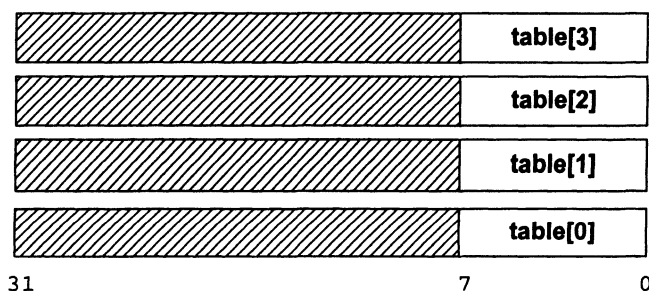
Figure 4-3: Unpacked arrays can store each element independently
