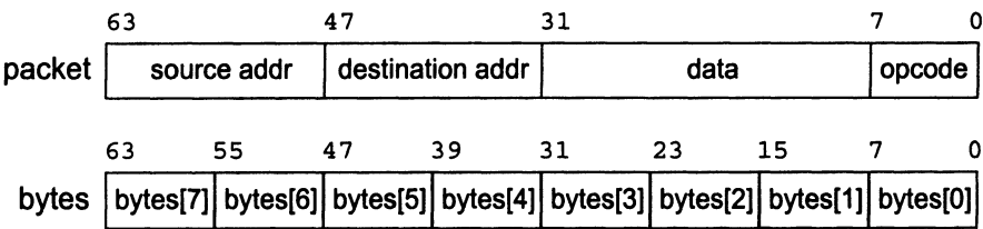
Figure 4-2: Packed union with two representations of the same storage
