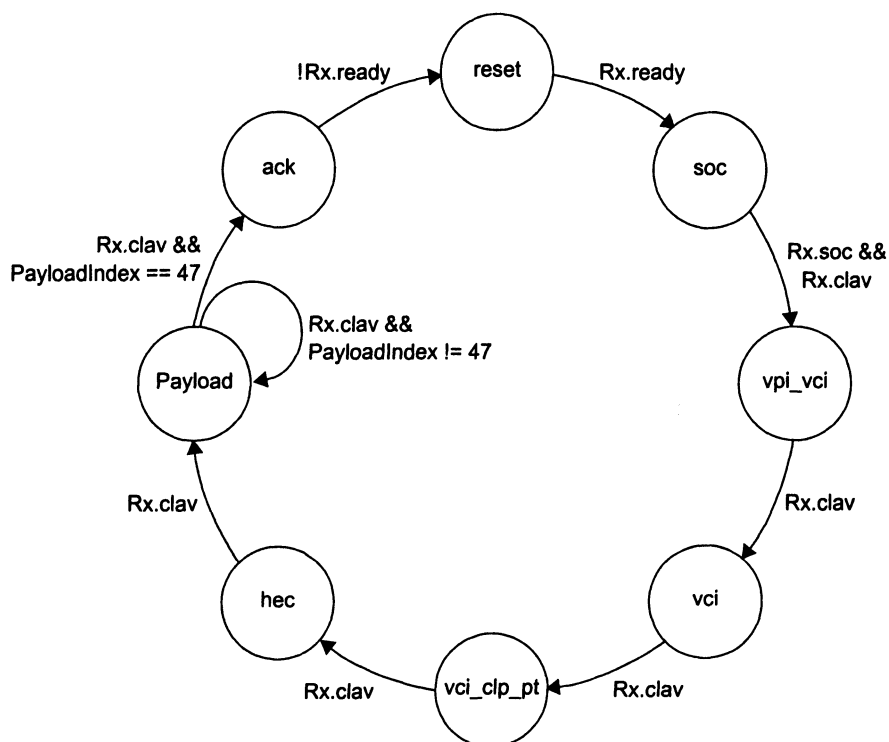
Figure 10-3: Receiver state flow diagram
